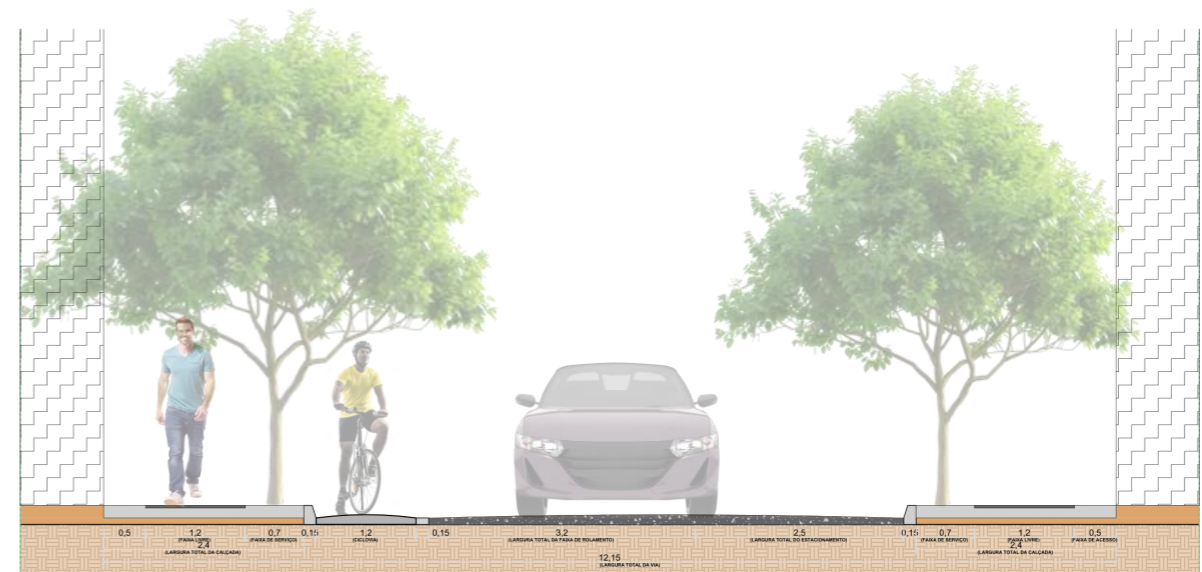
ESCALA 1:20 VIA COMPLETA - IDEAL
